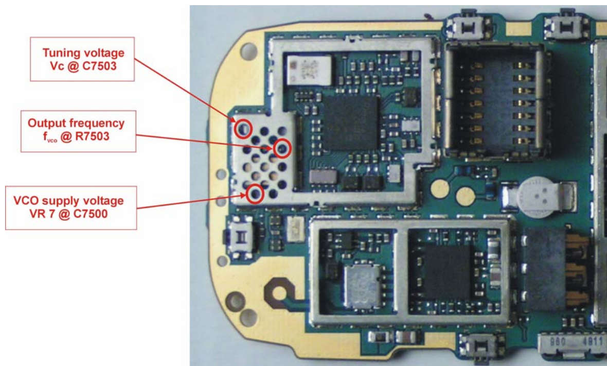
Figure 1: Test holes in the VCO chamber
